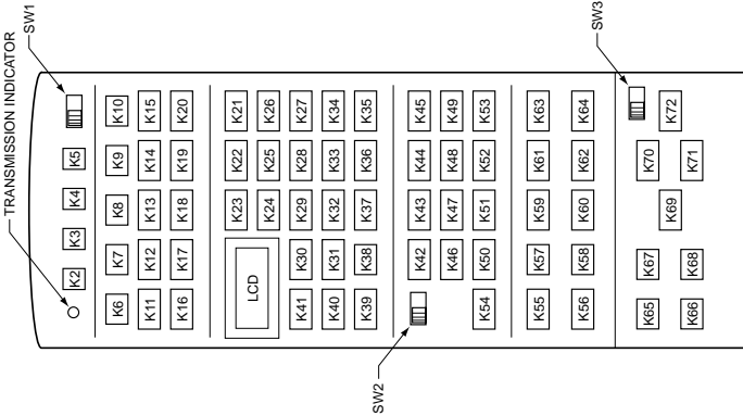
Key arrangement
